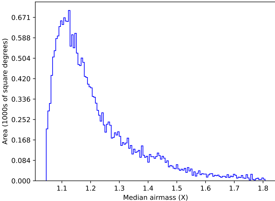
reweight_plane_v3.3_10yrs Yr 1 u band: Median airmass
