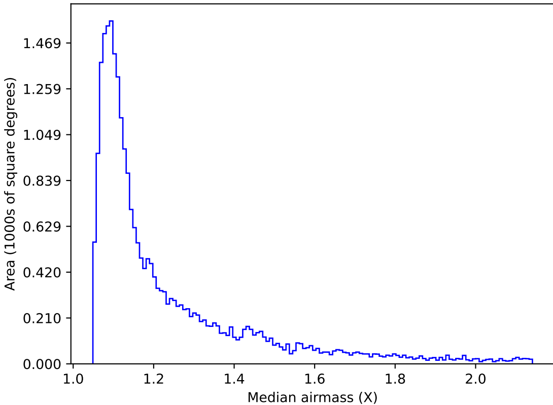
reweight_plane_v3.3_10yrs Yr 1 r band: Median airmass
