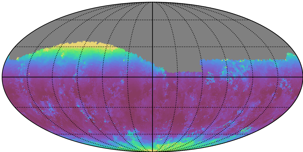
reweight_plane_v3.3_10yrs Yr 1 g band: Median airmass
