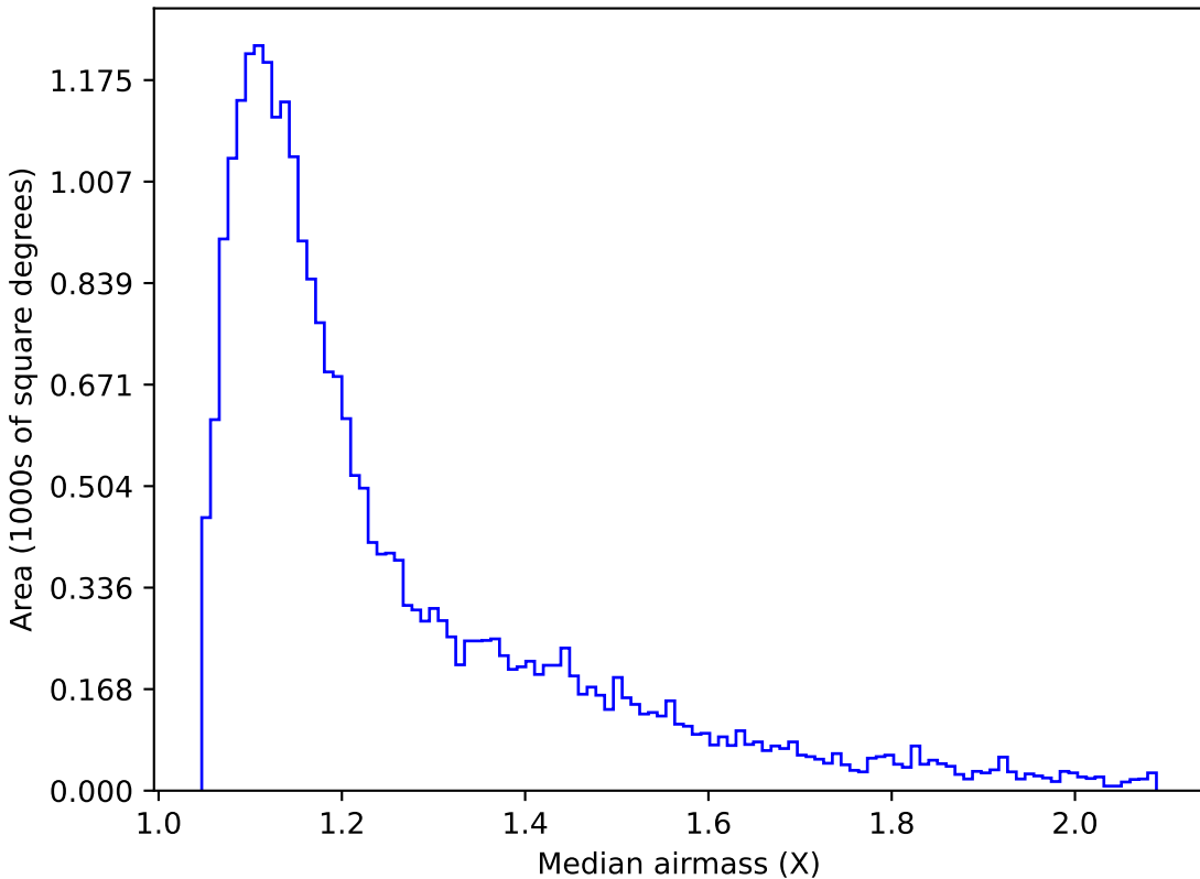
reweight_plane_v3.3_10yrs Yr 1 g band: Median airmass
