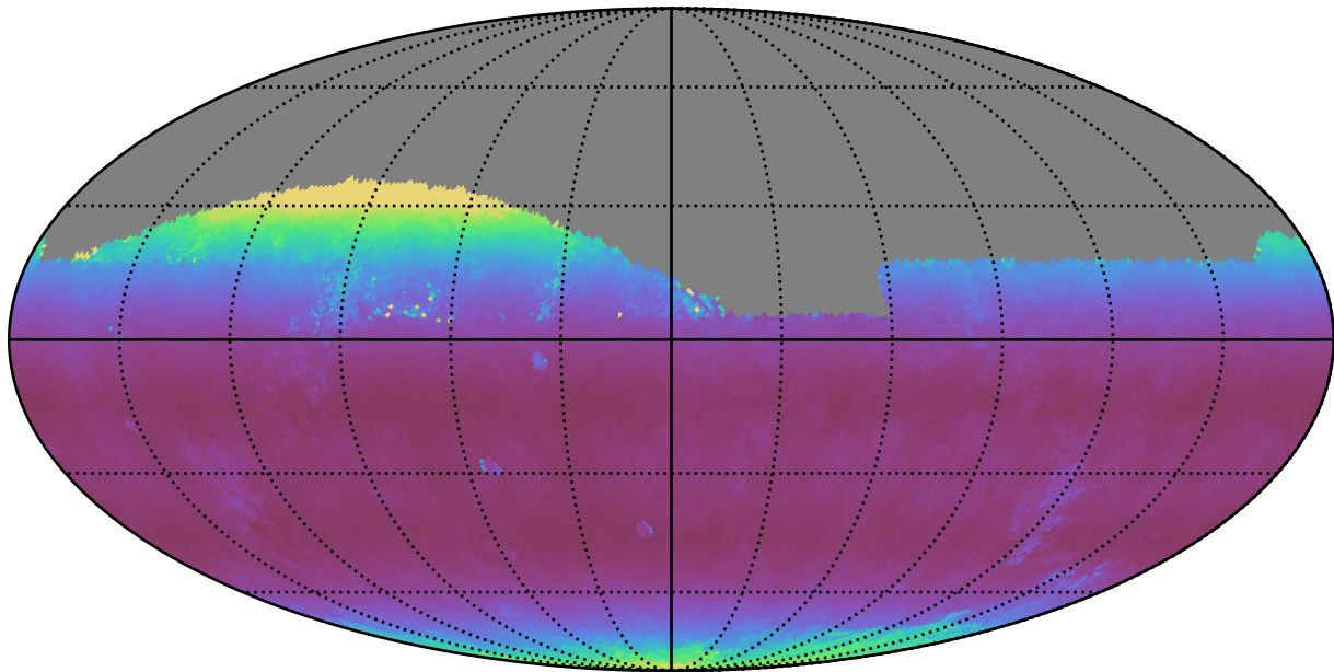
reweight_plane_v3.3_10yrs Yr 1 all bands: Median airmass
