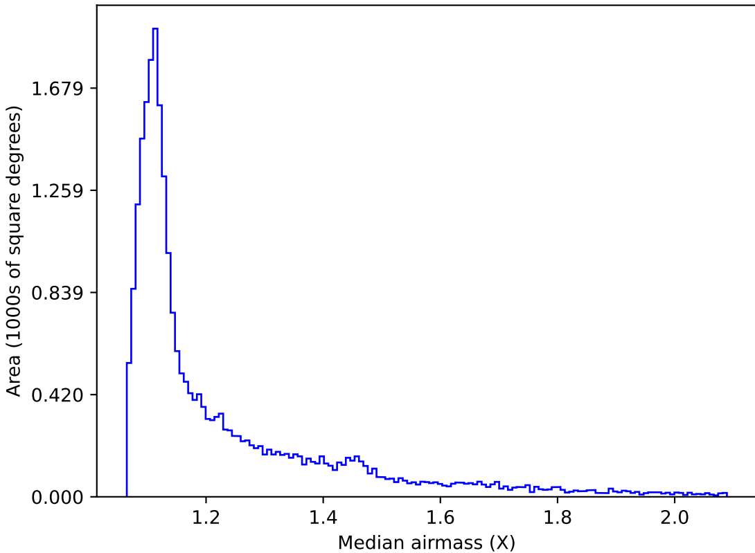
reweight_plane_v3.3_10yrs Yr 1 all bands: Median airmass
