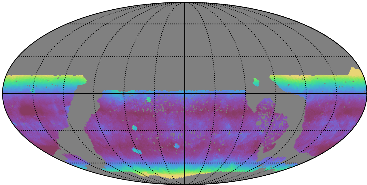
reweight_plane_v3.3_10yrs WFD z band: Median airmass
