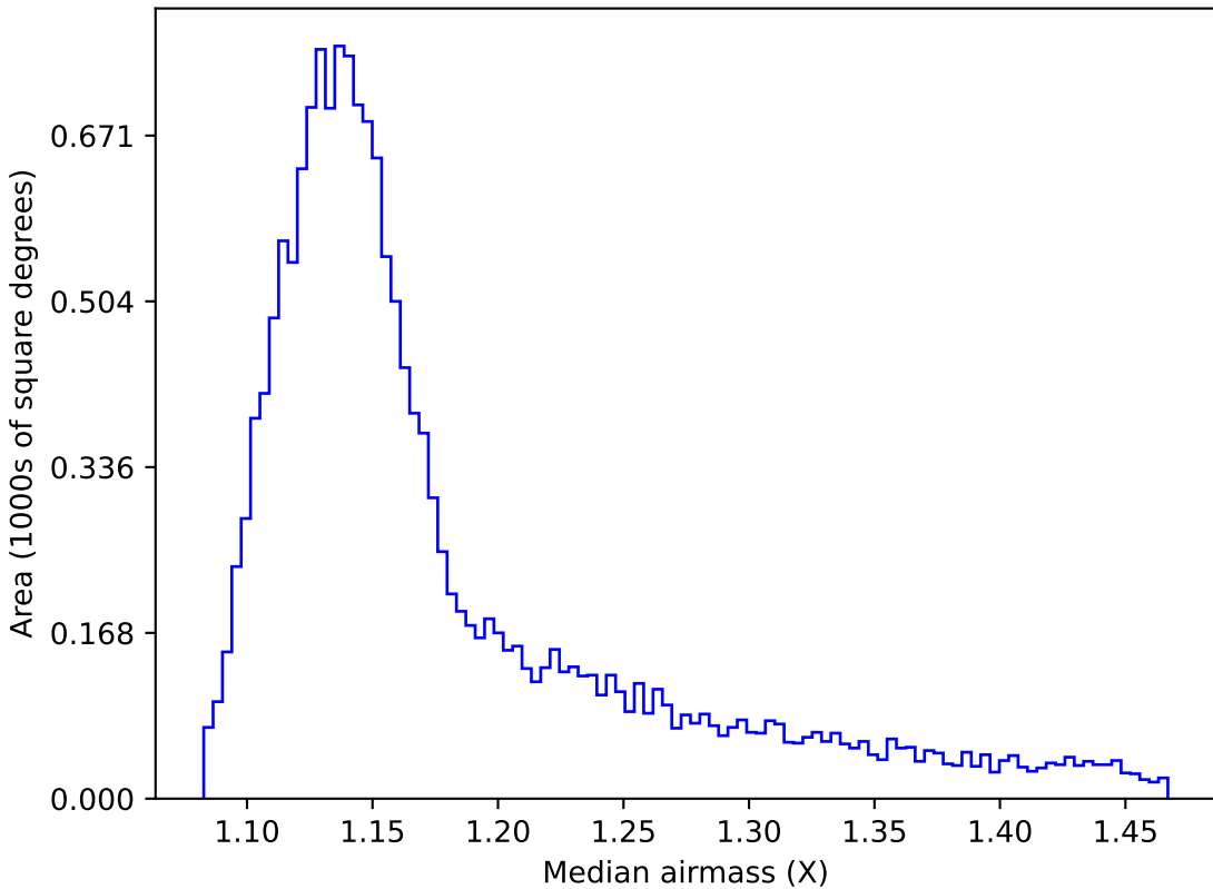
reweight_plane_v3.3_10yrs WFD z band: Median airmass
