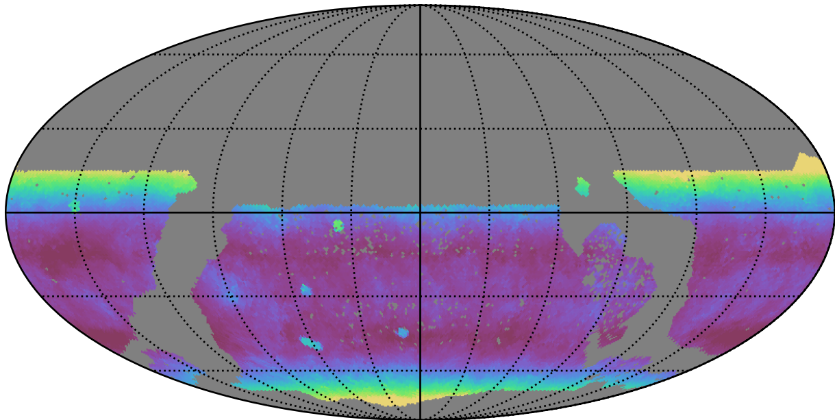
reweight_plane_v3.3_10yrs WFD y band: Median airmass
