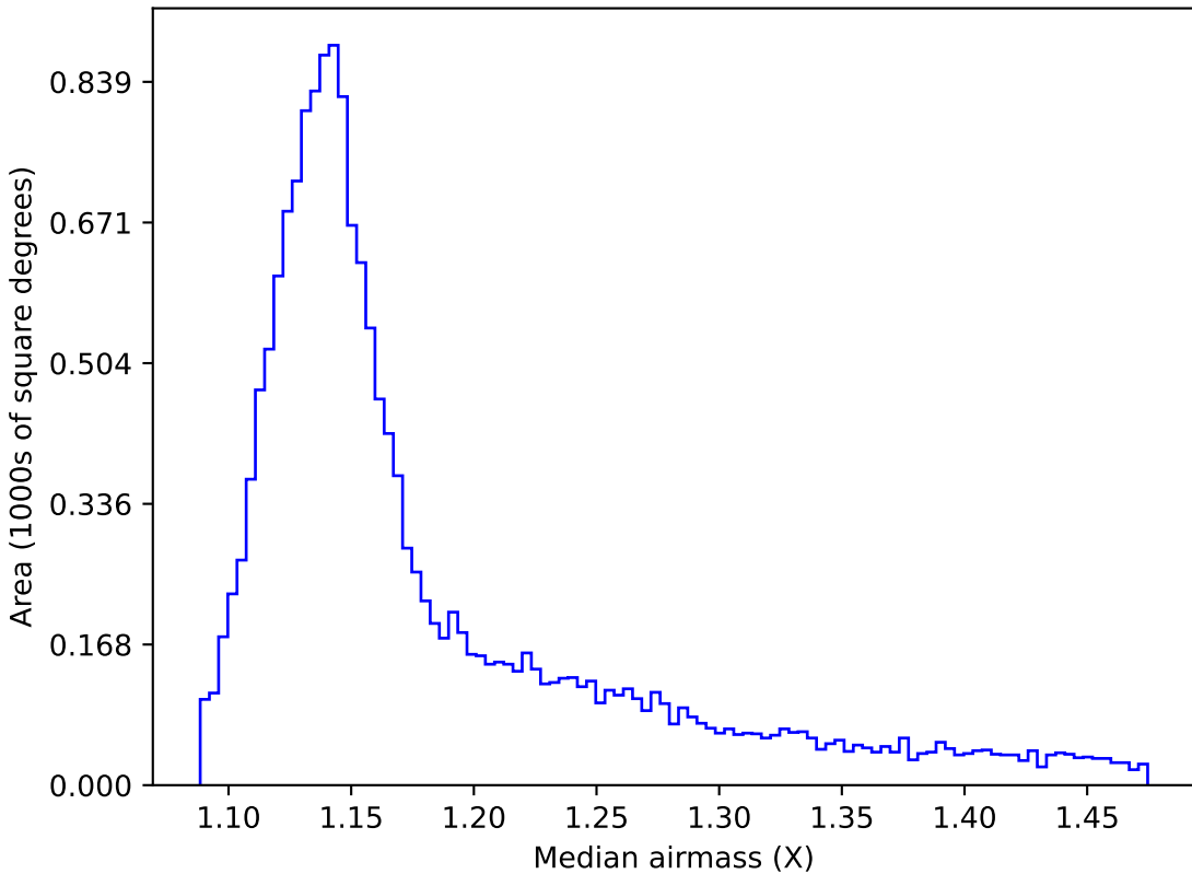
reweight_plane_v3.3_10yrs WFD y band: Median airmass
