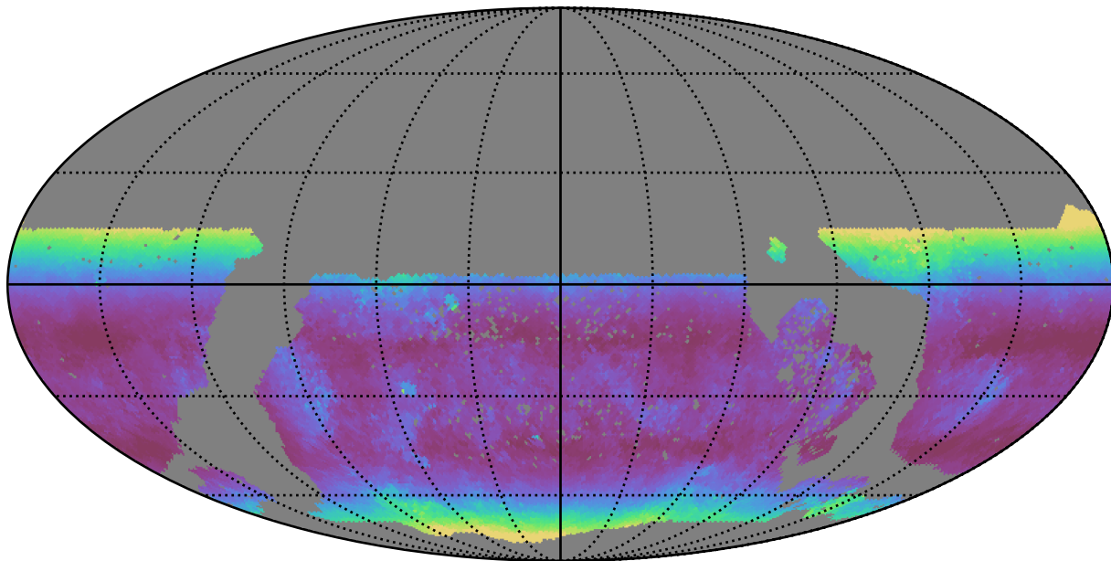
reweight_plane_v3.3_10yrs WFD u band: Median airmass
