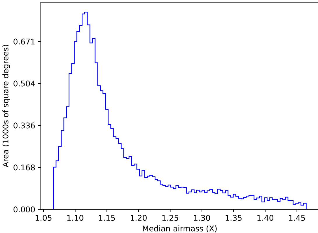
reweight_plane_v3.3_10yrs WFD u band: Median airmass
