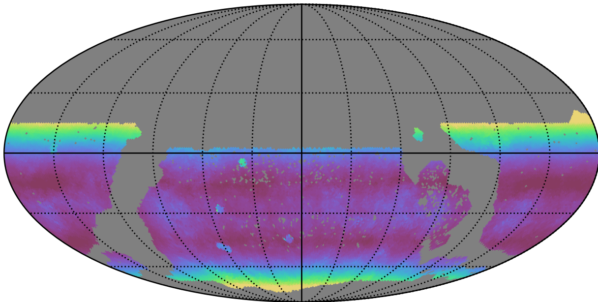
reweight_plane_v3.3_10yrs WFD r band: Median airmass
