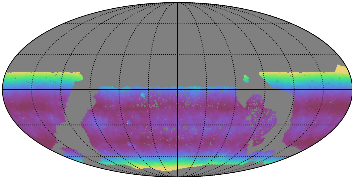
reweight_plane_v3.3_10yrs WFD i band: Median airmass
