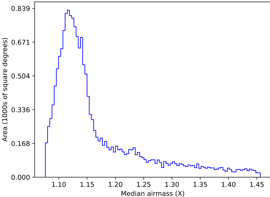
reweight_plane_v3.3_10yrs WFD i band: Median airmass
