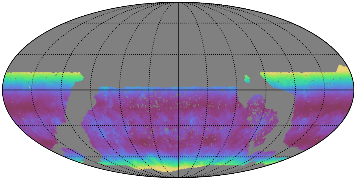
reweight_plane_v3.3_10yrs WFD g band: Median airmass
