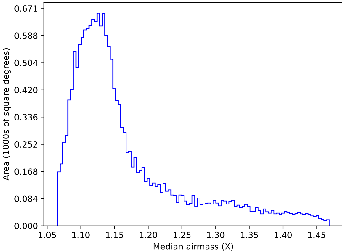
reweight_plane_v3.3_10yrs WFD g band: Median airmass
