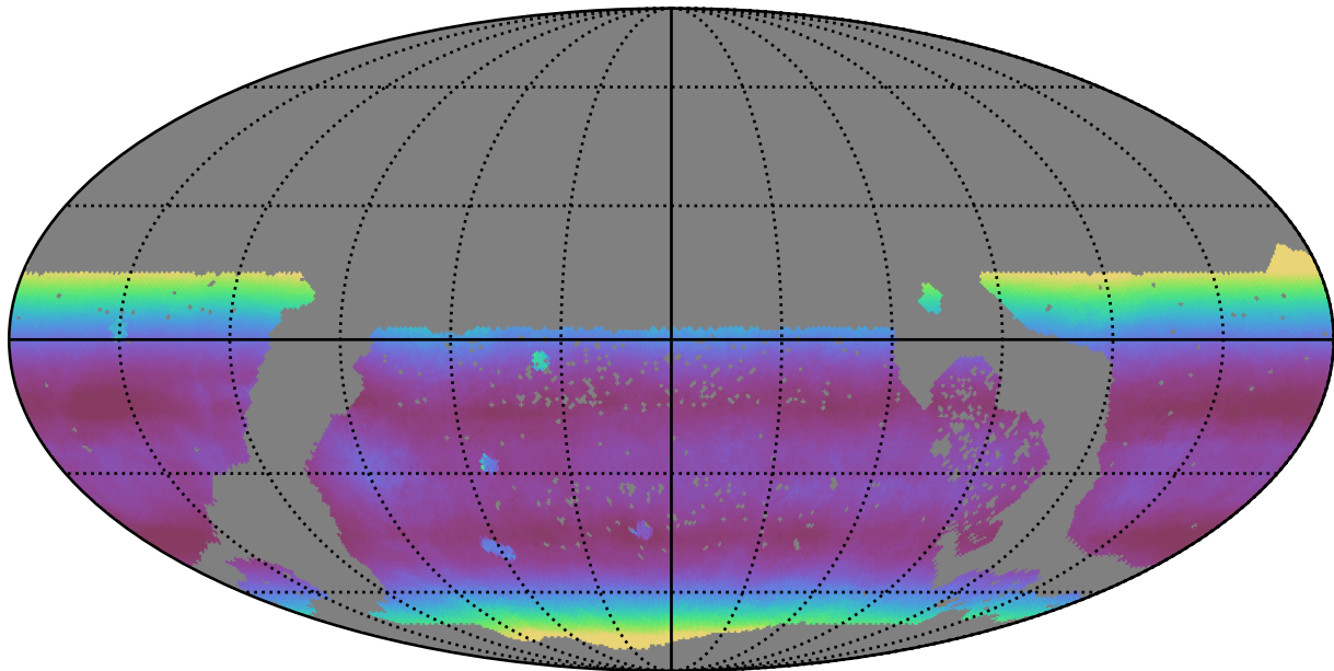
reweight_plane_v3.3_10yrs WFD all bands: Median airmass
