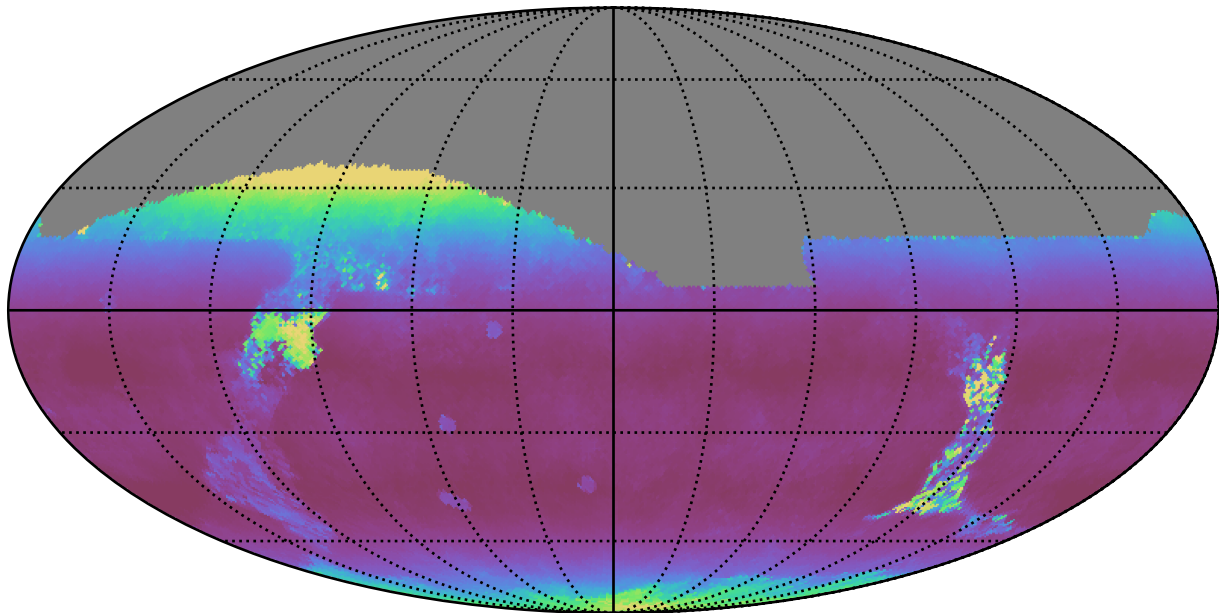
reweight_plane_v3.3_10yrs All sky z band: Median airmass
