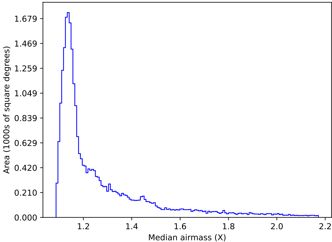
reweight_plane_v3.3_10yrs All sky z band: Median airmass
