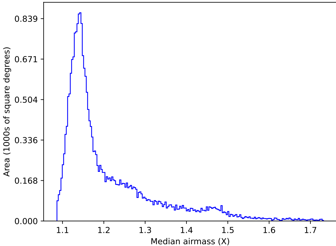
reweight_plane_v3.3_10yrs All sky y band: Median airmass
