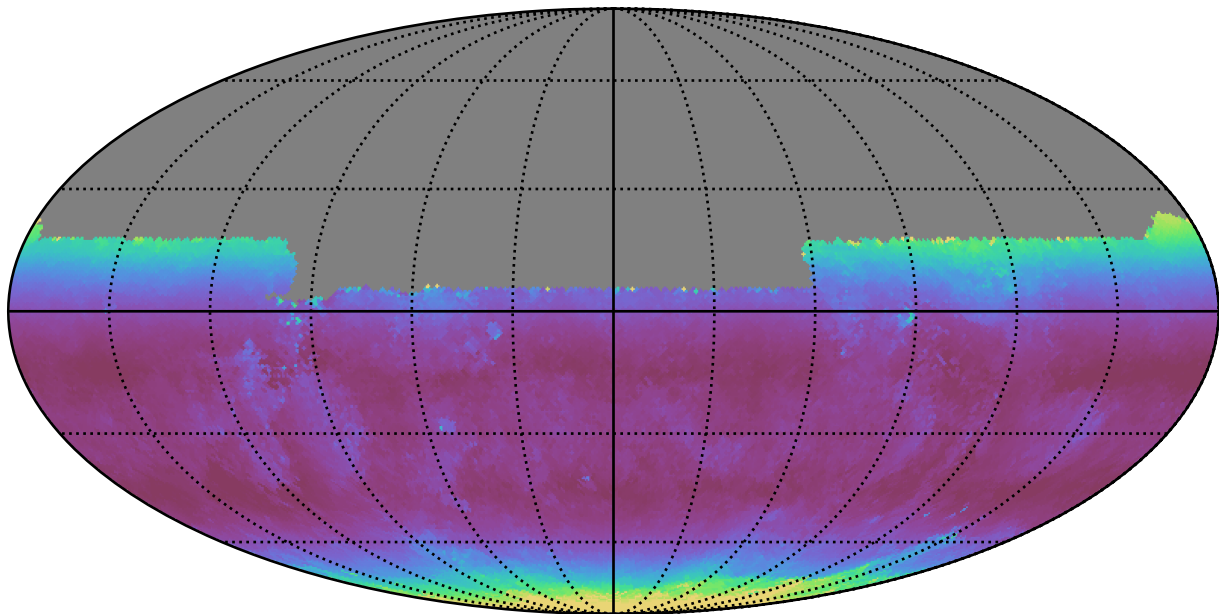
reweight_plane_v3.3_10yrs All sky u band: Median airmass
