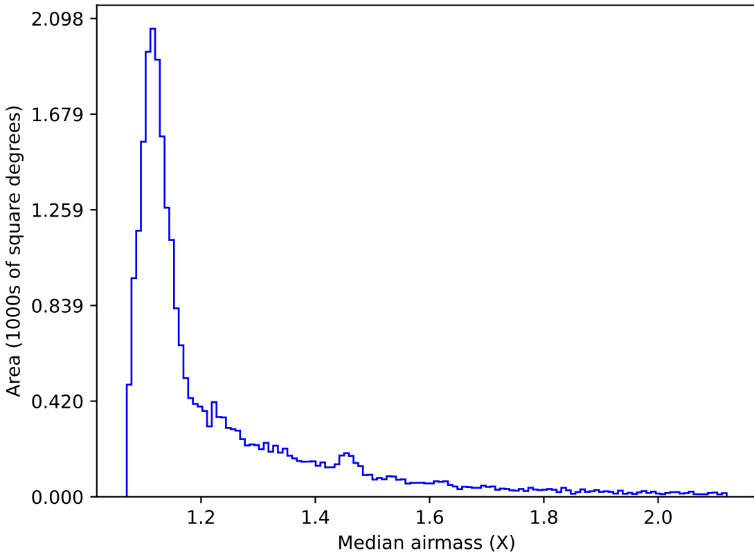
reweight_plane_v3.3_10yrs All sky r band: Median airmass
