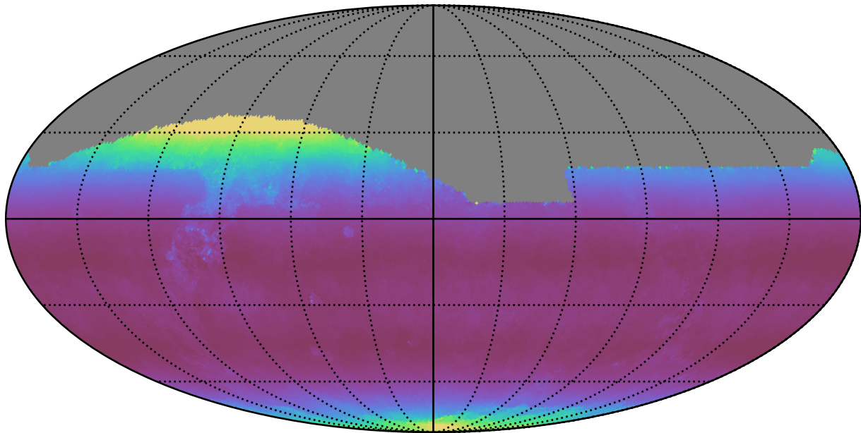
reweight_plane_v3.3_10yrs All sky i band: Median airmass
