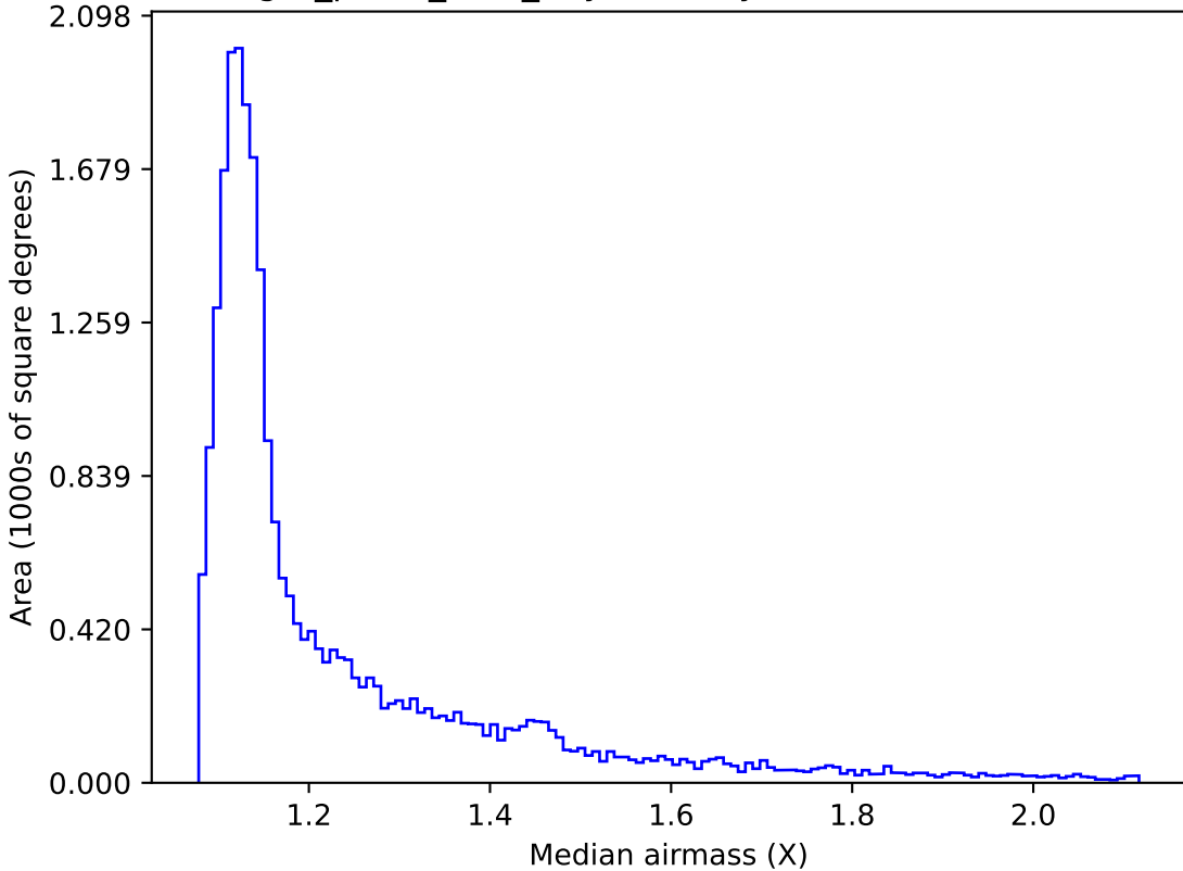
reweight_plane_v3.3_10yrs All sky i band: Median airmass
