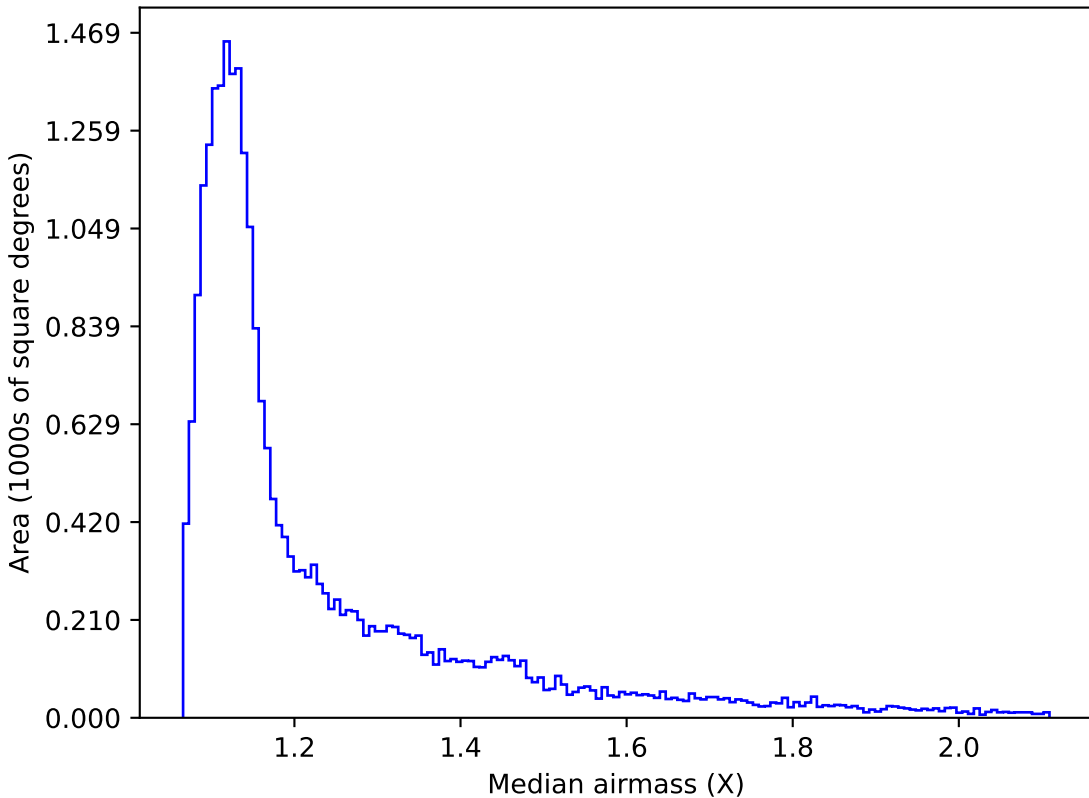
reweight_plane_v3.3_10yrs All sky g band: Median airmass
