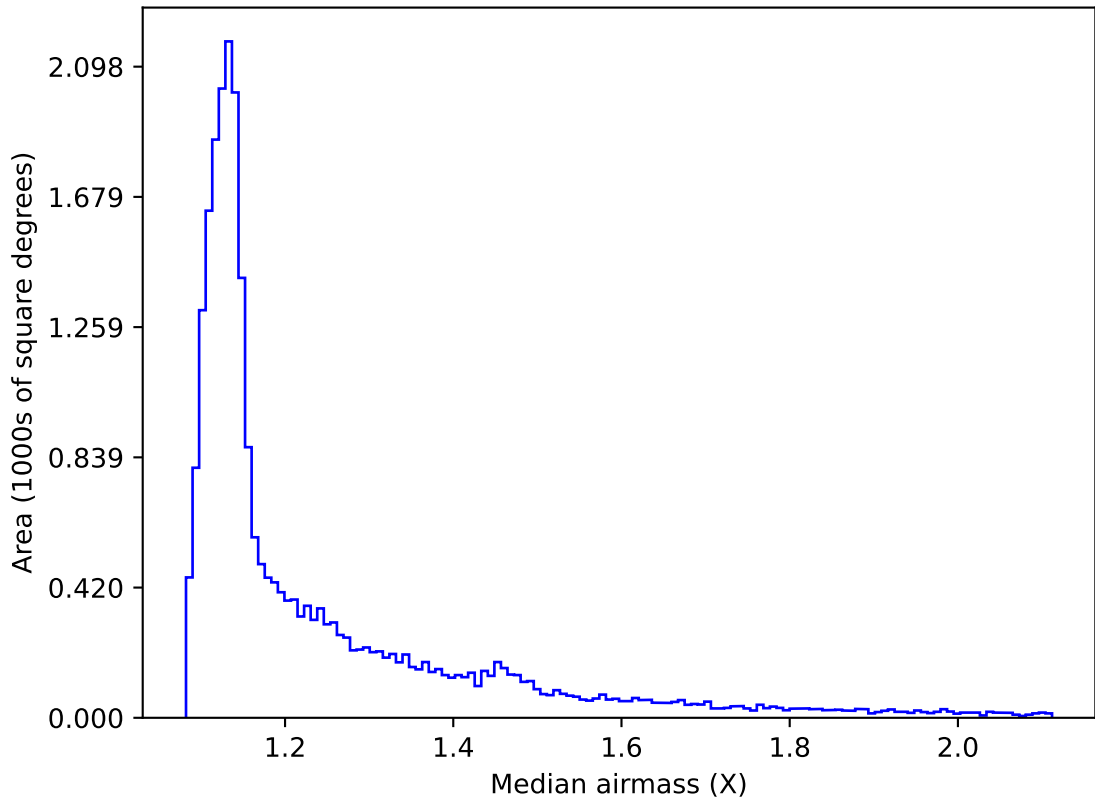
reweight_plane_v3.3_10yrs All sky all bands: Median airmass
