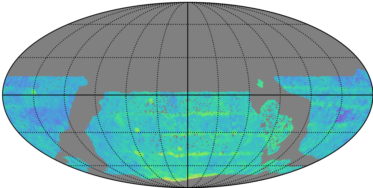
reweight_plane_v3.3_10yrs WFD z band: Median Season Length
