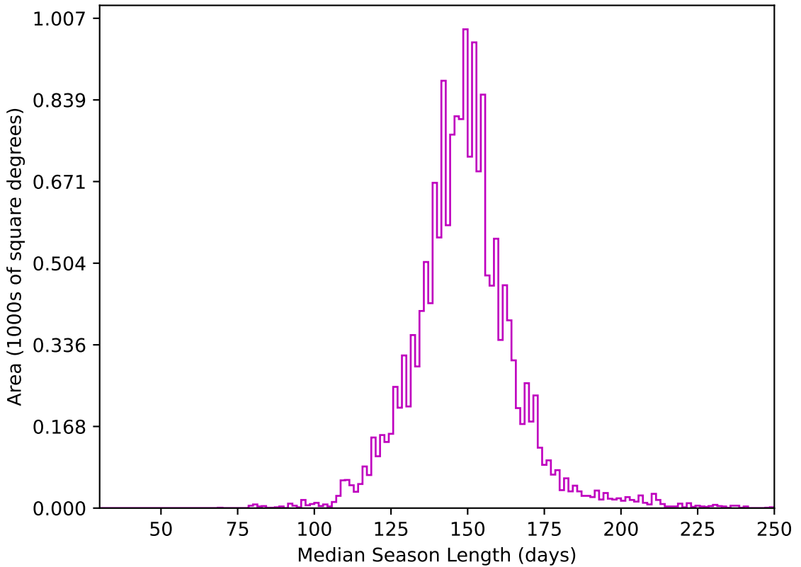
reweight_plane_v3.3_10yrs WFD z band: Median Season Length
