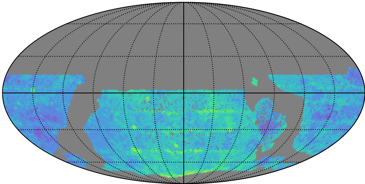
reweight_plane_v3.3_10yrs WFD y band: Median Season Length
