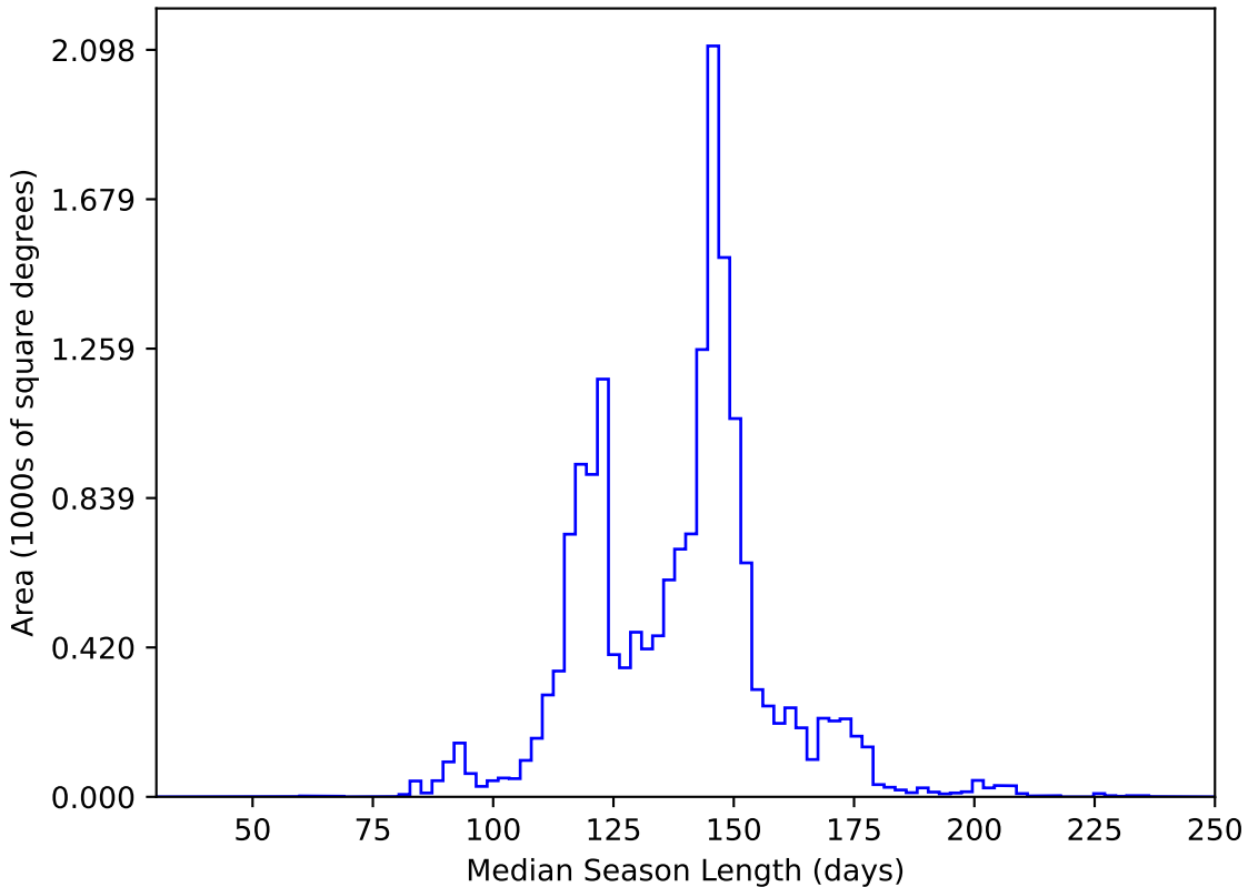
reweight_plane_v3.3_10yrs WFD y band: Median Season Length
