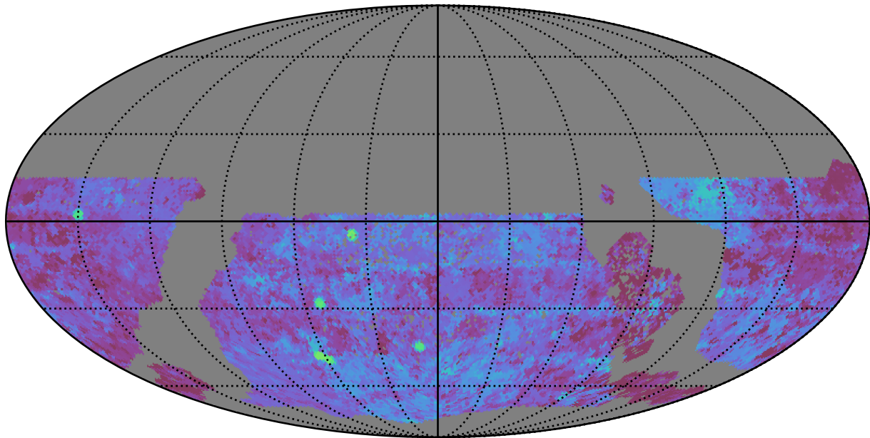
reweight_plane_v3.3_10yrs WFD u band: Median Season Length
