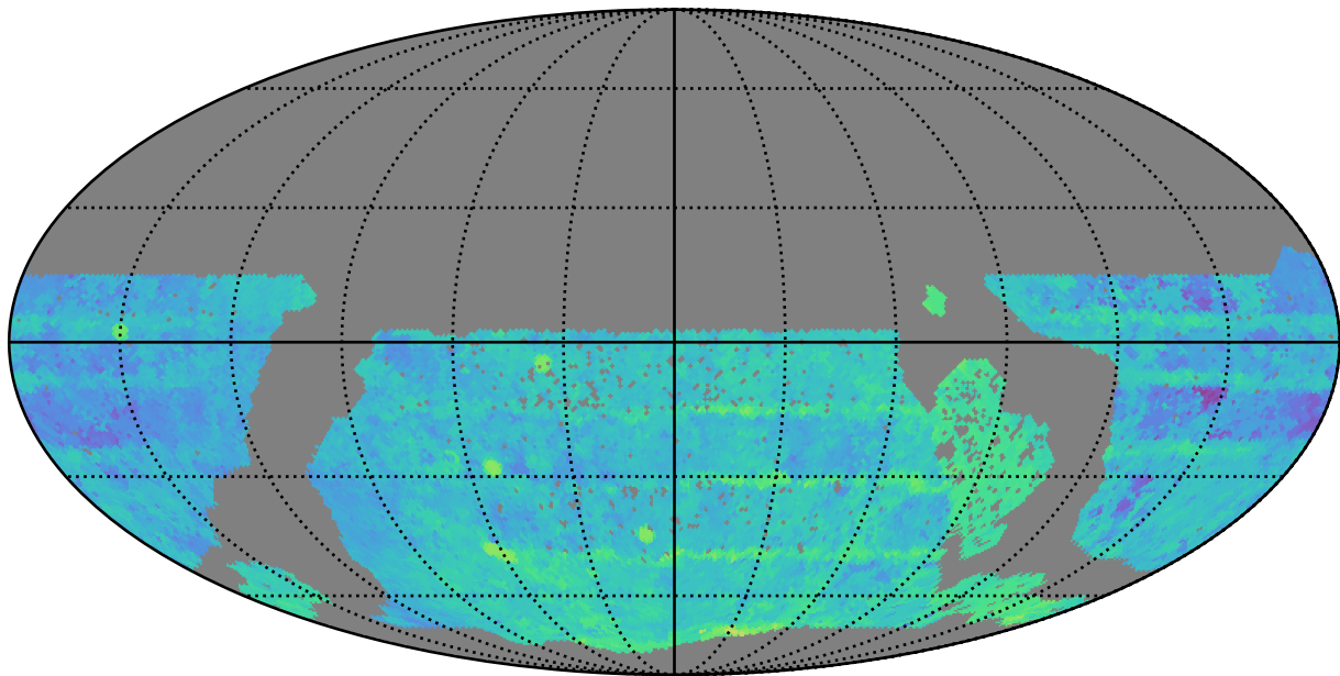
reweight_plane_v3.3_10yrs WFD r band: Median Season Length
