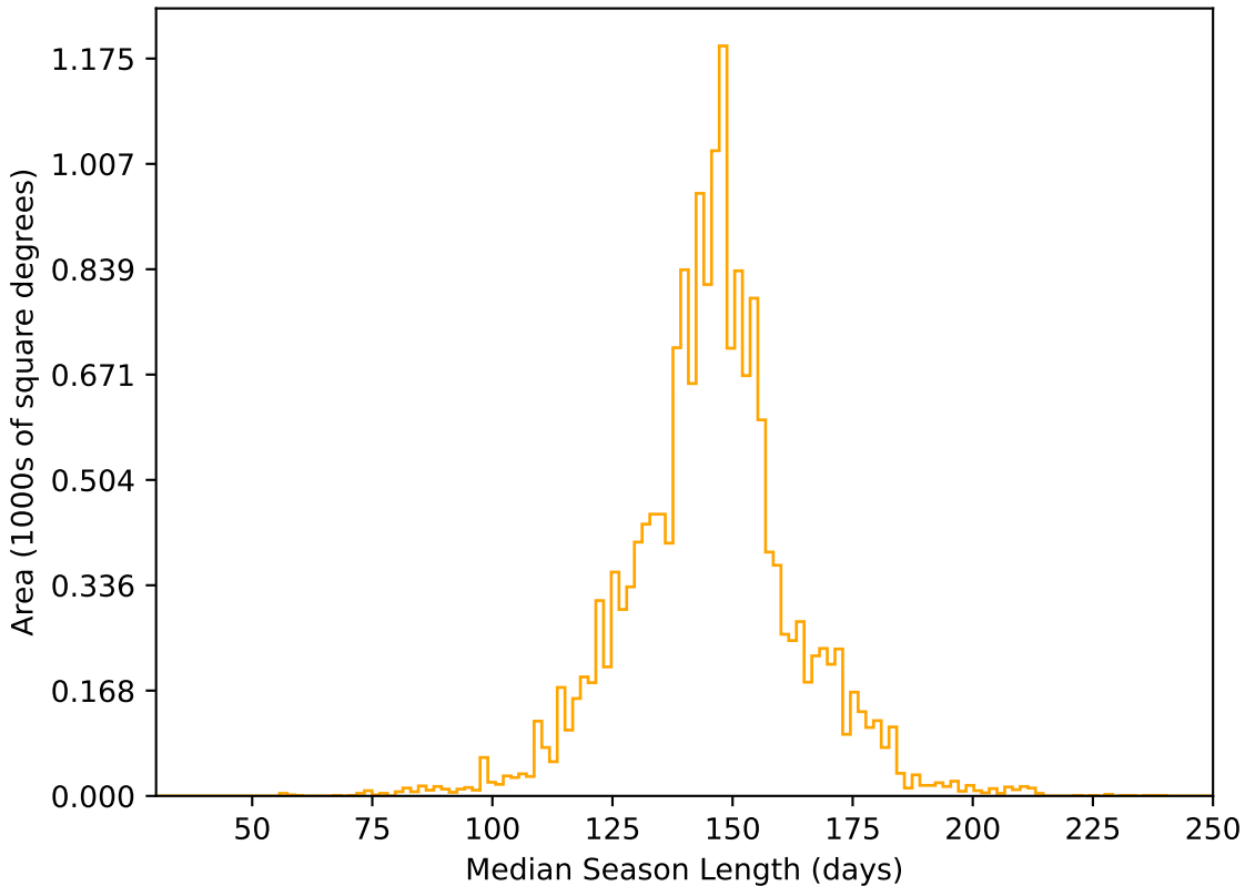
reweight_plane_v3.3_10yrs WFD r band: Median Season Length
