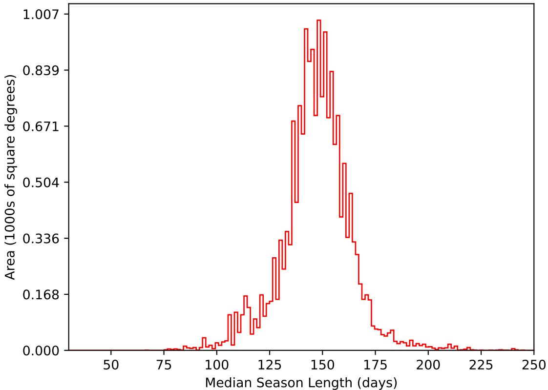
reweight_plane_v3.3_10yrs WFD i band: Median Season Length
