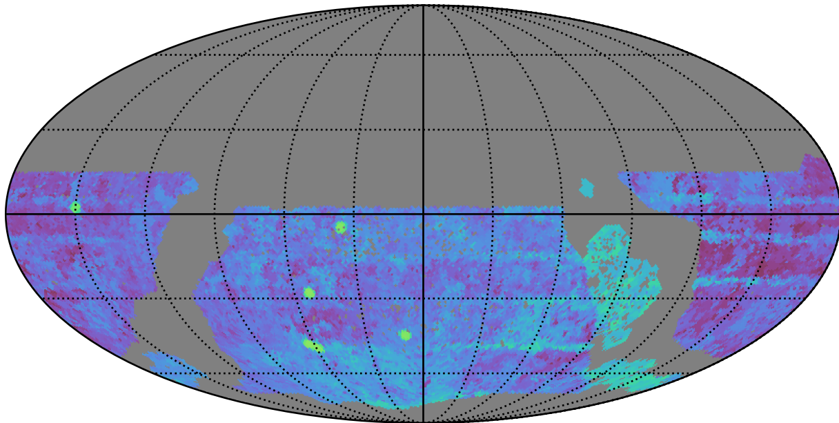
reweight_plane_v3.3_10yrs WFD g band: Median Season Length
