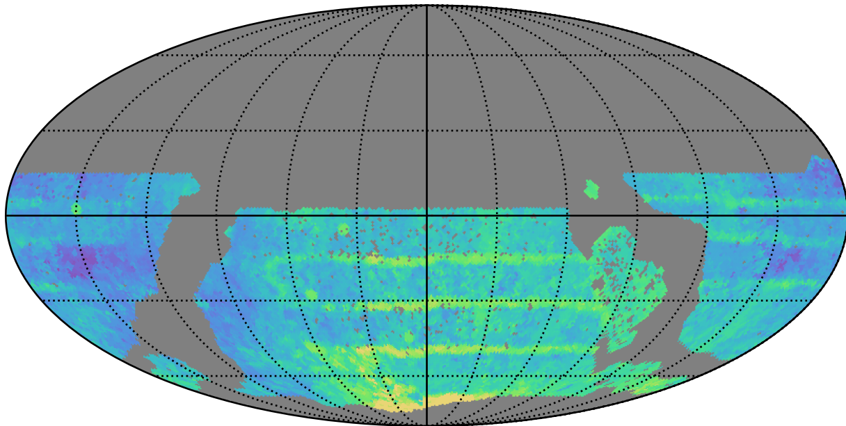
reweight_plane_v3.3_10yrs WFD all bands: Median Season Length
