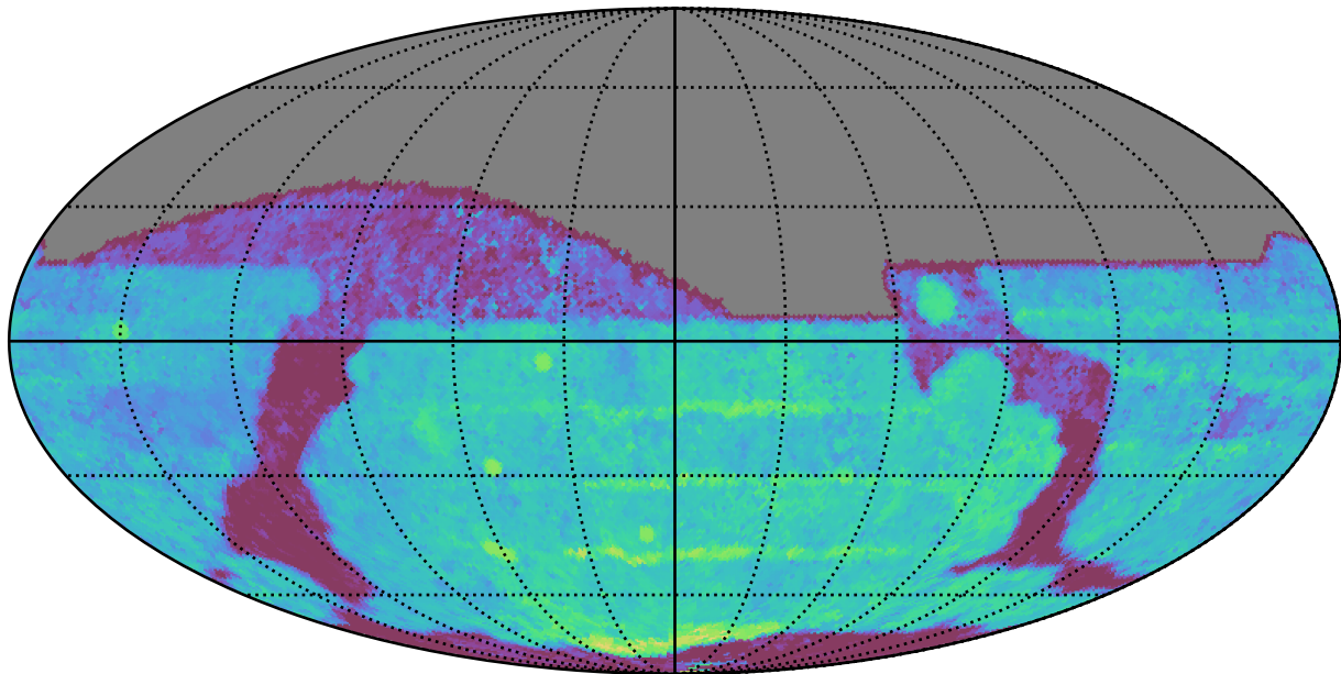
reweight_plane_v3.3_10yrs All sky z band: Median Season Length
