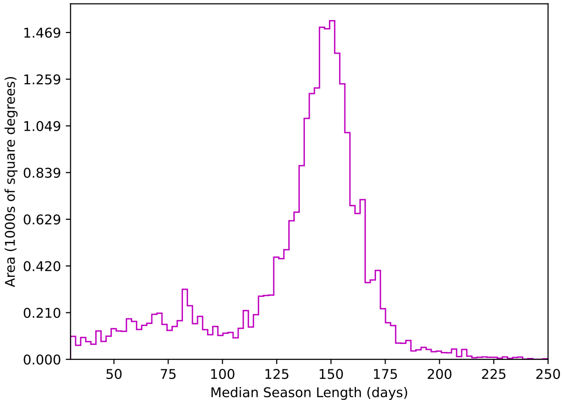
reweight_plane_v3.3_10yrs All sky z band: Median Season Length
