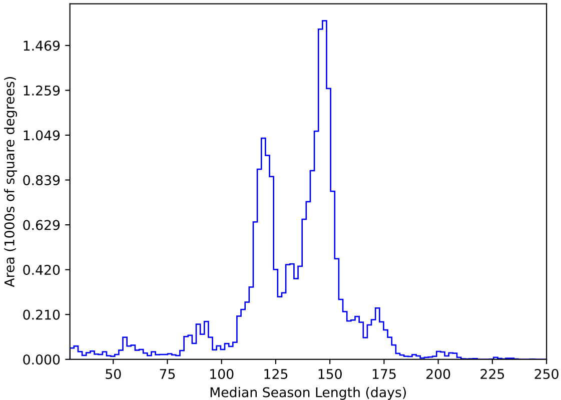
reweight_plane_v3.3_10yrs All sky y band: Median Season Length
