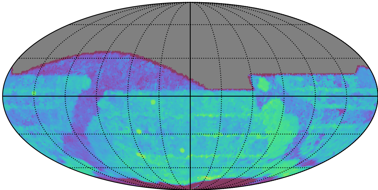
reweight_plane_v3.3_10yrs All sky r band: Median Season Length
