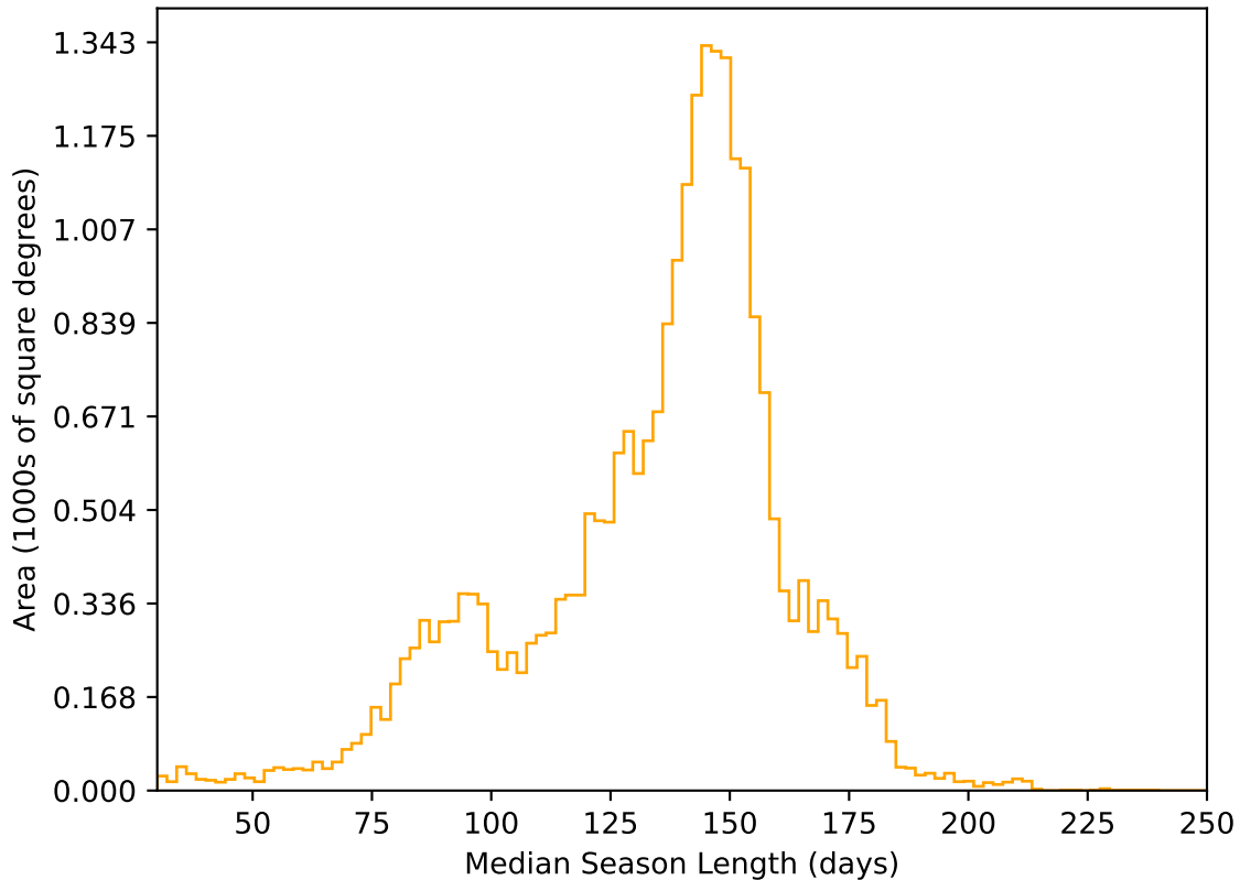
reweight_plane_v3.3_10yrs All sky r band: Median Season Length
