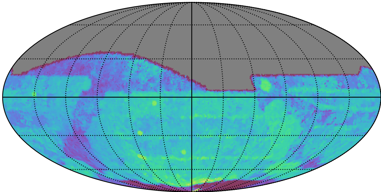
reweight_plane_v3.3_10yrs All sky i band: Median Season Length
