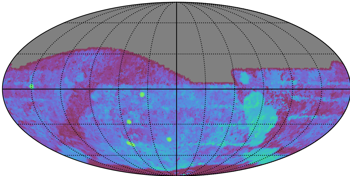
reweight_plane_v3.3_10yrs All sky g band: Median Season Length
