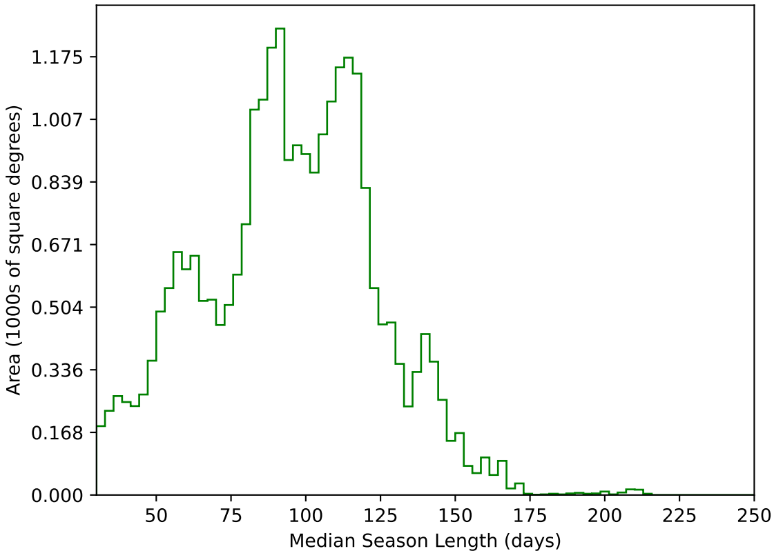
reweight_plane_v3.3_10yrs All sky g band: Median Season Length
