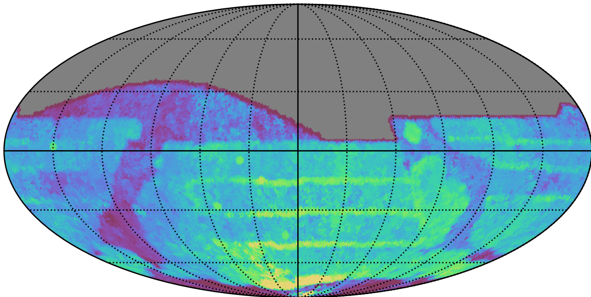
reweight_plane_v3.3_10yrs All sky all bands: Median Season Length
