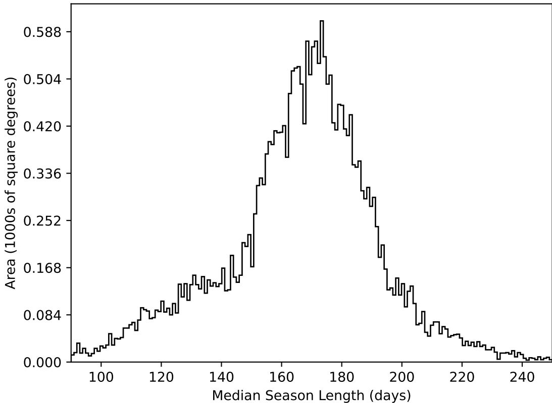
reweight_plane_v3.3_10yrs All sky all bands: Median Season Length
