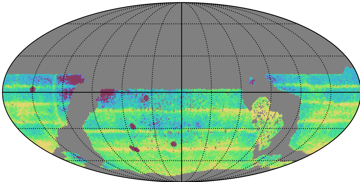
reweight_plane_v3.3_10yrs WFD: Median Intra-Night Gap
