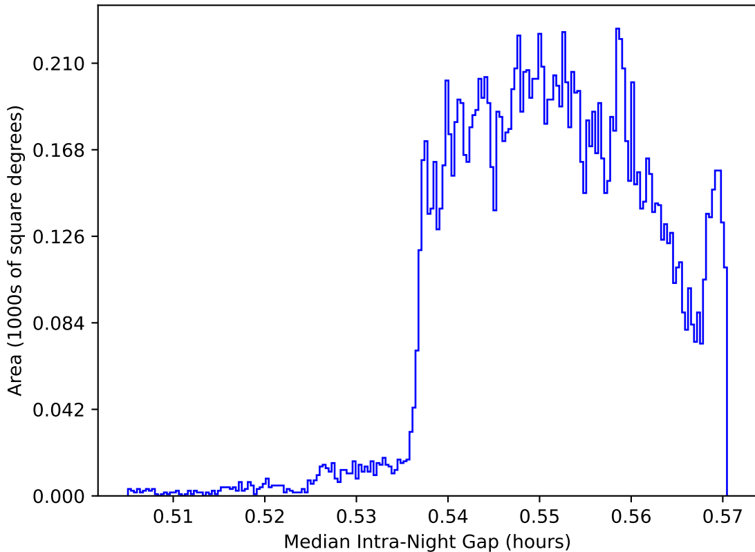
reweight_plane_v3.3_10yrs WFD: Median Intra-Night Gap
