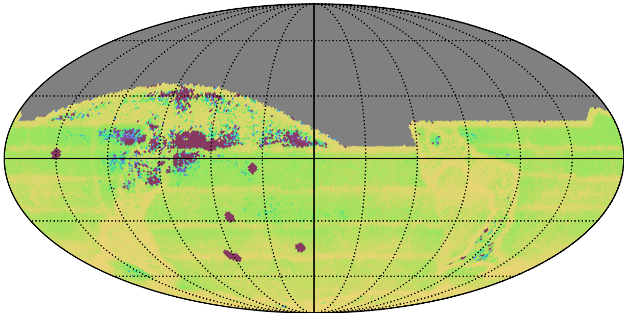
reweight_plane_v3.3_10yrs All sky: Median Intra-Night Gap
